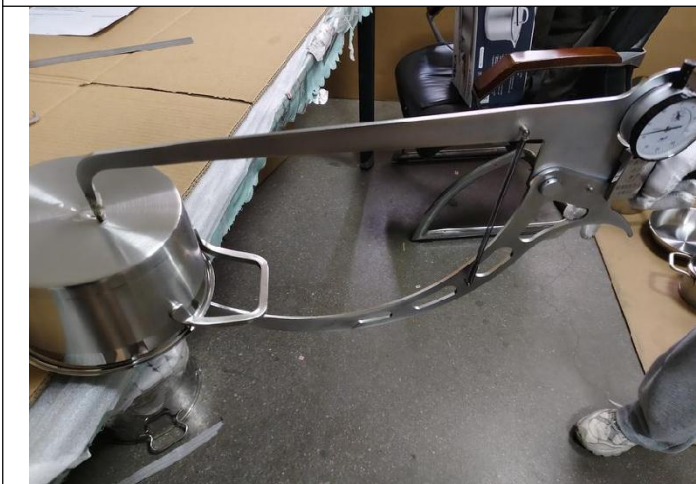
Size check
