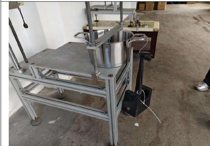
Load-bearing test
