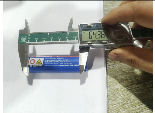
Printing size:64.36mm
