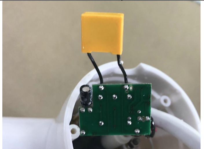
Internal view
