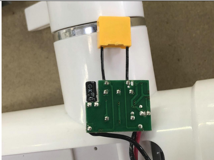
Internal view
