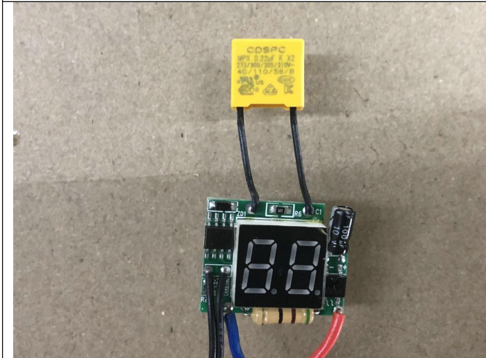
Internal view
