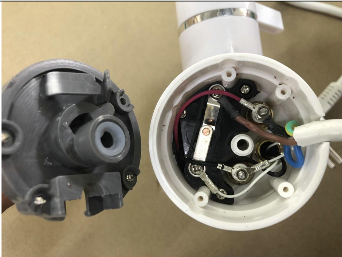
Internal view
