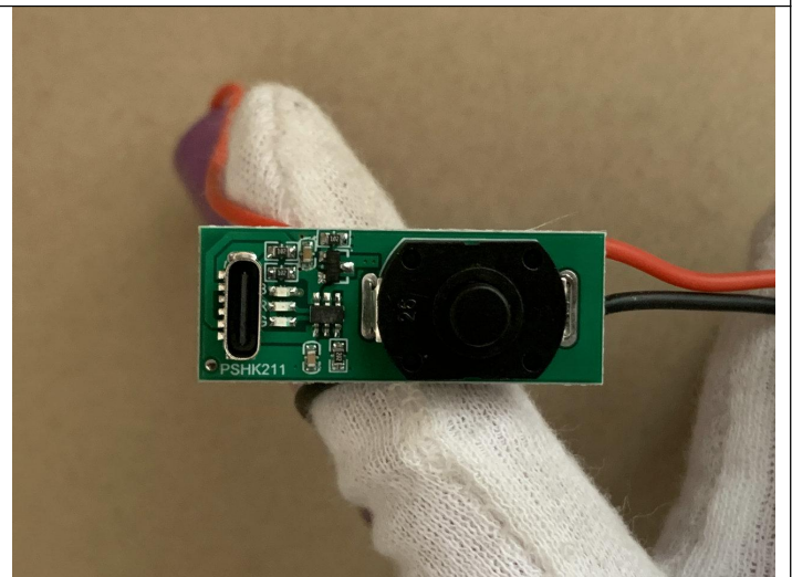
Internal view
