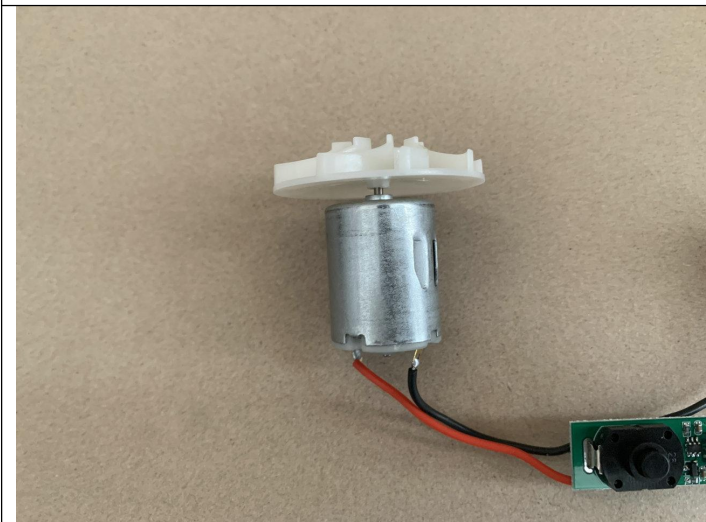
Internal view
